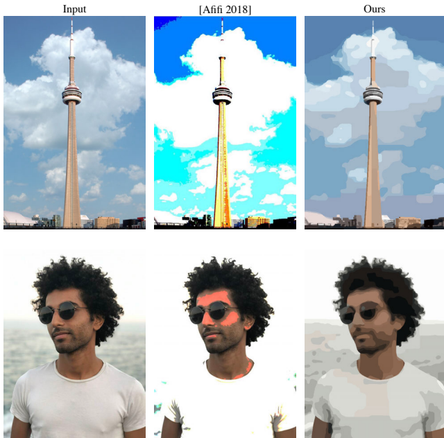
Figure 15: Our algorithm generates posterizations with smooth boundaries and accurate colors (and can be recolored). The bilateral filtering technique creates overexposed colors with noisier boundaries. ©Omar Abdelaal.
